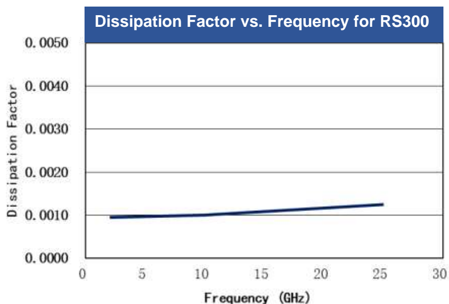
Figure 2 Demonstrates the Stability of Dissipation Factor across Frequency. This characteristic demonstrates the inherent robustness of Relong Laminates across Frequency, providing a stable platform for high frequency applications where signal integrity is critical to the overall performance of the application.
