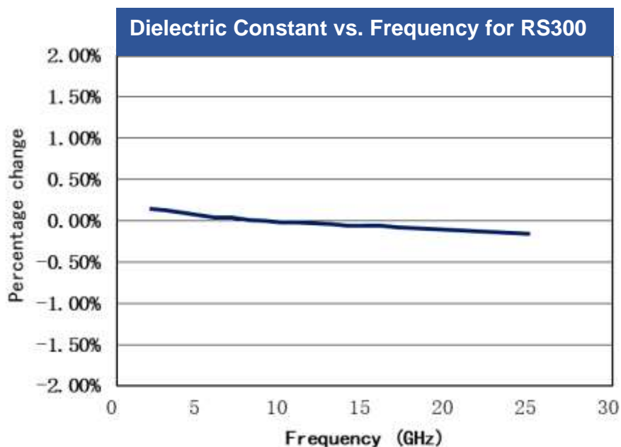
Figure 1 Demonstrates the Stability of Dielectric Constant across Frequency. This characteristic demonstrates the inherent robustness of Relong Laminates across Frequency, thus simplifying the final design process when working across EM spectrum. The stability of the Dielectric Constant of RS300 over frequency ensures easy design transition and scalability of design.
